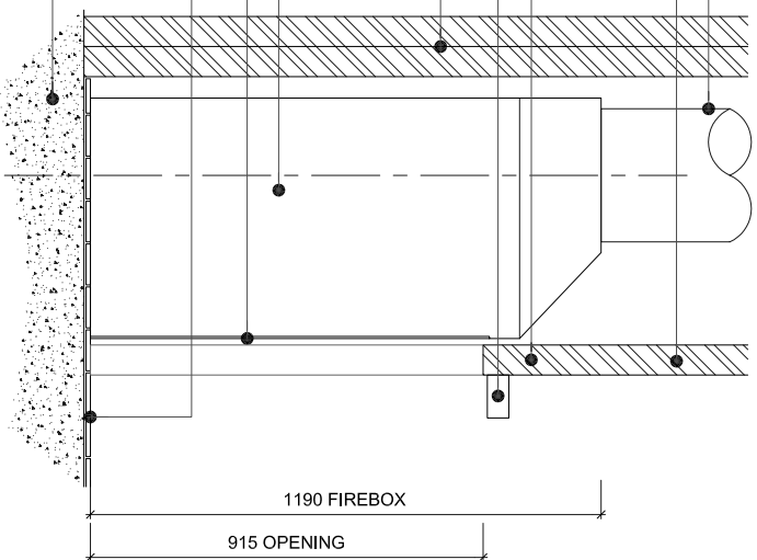
3 SIDE ELEVATION B900 SCALE 1:20
