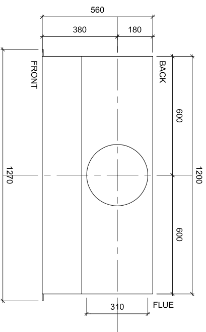
1 PLAN Z1200 SCALE 1:20
