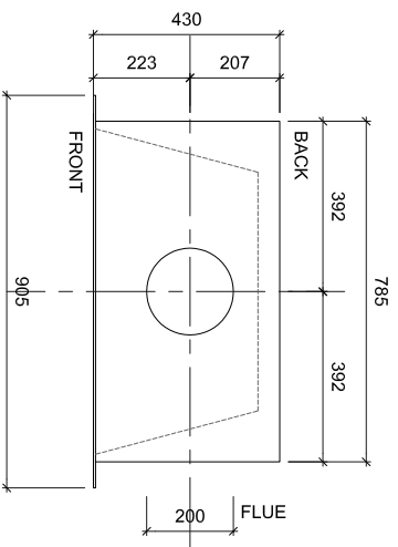
1 PLAN
